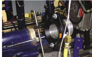
A Model 120024 4" (102mm) Super Air Amplifier cools an engine during dynamometer testing.
