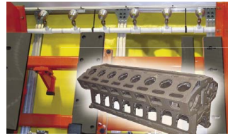
A series of Model 6042 2" (51mm) Adjustable Air Amplifiers blow coolant off 16 cylinder diesel engines.
