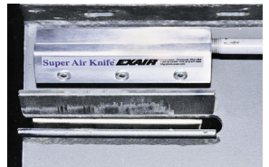
With a 40:1 air amplification ratio, a high volume of airflow is the result from minimal air input to keep linear induction motors from overheating.
